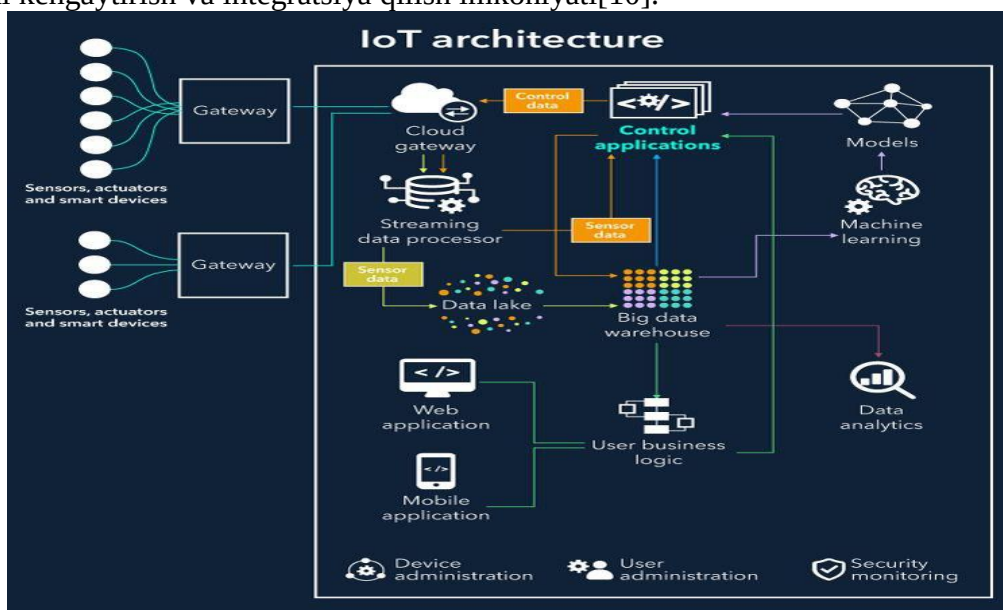
1-rasm. IoT tizimining strukturalari
