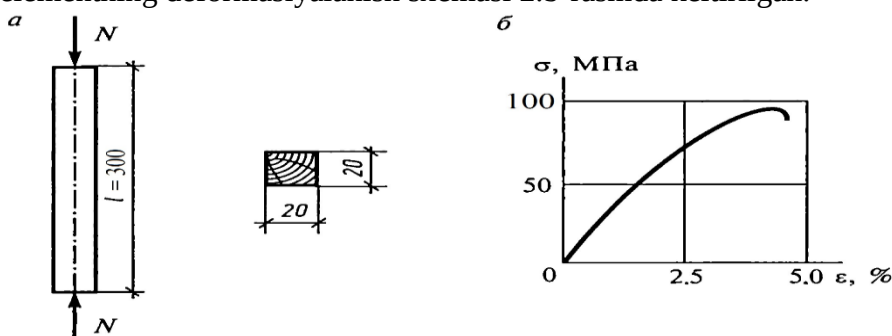
2-rasm. a) standart namuna; b) bo‘ylama kuchlanish va deformasiyaning bog‘lanish diagrammasi.
