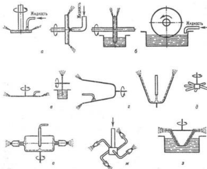
1-rasm. Mexanik zarrachalagichlar
