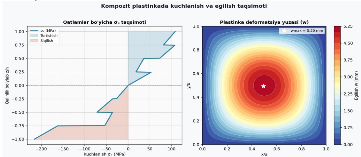
2-rasm. Plastinkada kuchlanish taqsimoti qatlamlar bo'yicha (chap) va deformatsiya yuzasi w(x,y) konturli ko'rinishi (o'ng)
